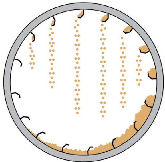
The diagram above illustrates how flights create the curtain in a rotary dryer to maximize heat transfer.
